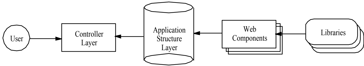
Figure 1. Structure of a READABLE Application
