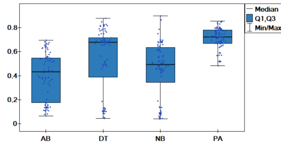
Fig. 3. Comparison of the results obtained for the four approaches: the baseline approach with algorithms AdaBoost, Decision Tree, Naive Bayes and the proposed approach.
