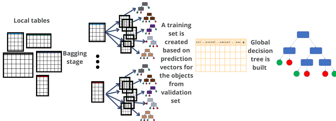
Fig. 1. Stages of model building.
