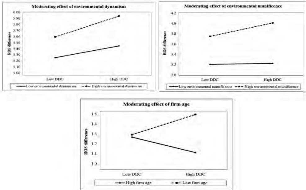
Figure 3: Interaction plots of the significant moderating effects
