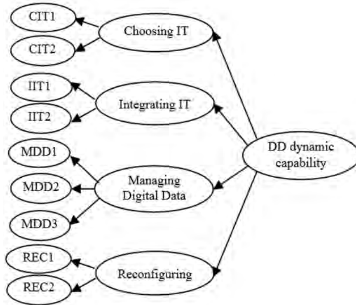
Figure 2: DD dynamic capability as a second-order construct
