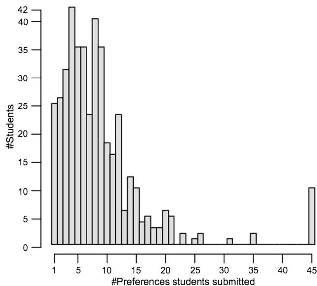
Fig. 2 Histogram of number of preferences of the students in the second field experiment
