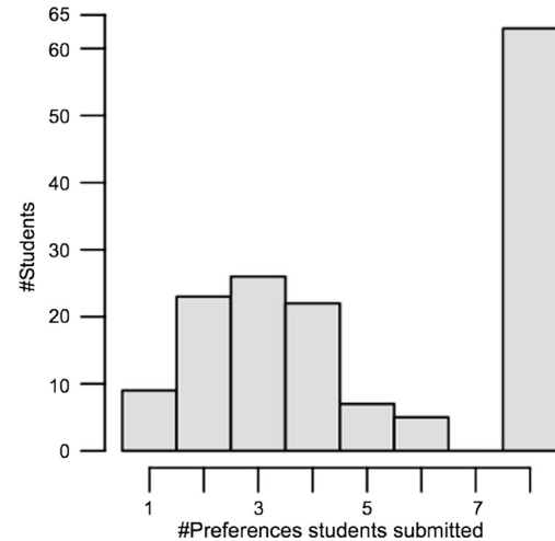
Fig. 1 Histogram of number of preferences of the students in the first field experiment
