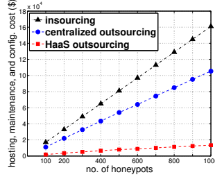
Figure 8. Expected cost for various honeypot deployment models
