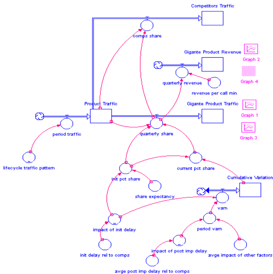
Figure 1: Stock and Flow model of impact of delays on market share and revenue
