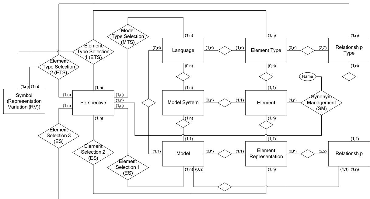
Figure 5: Configurative information modelling tool data model
