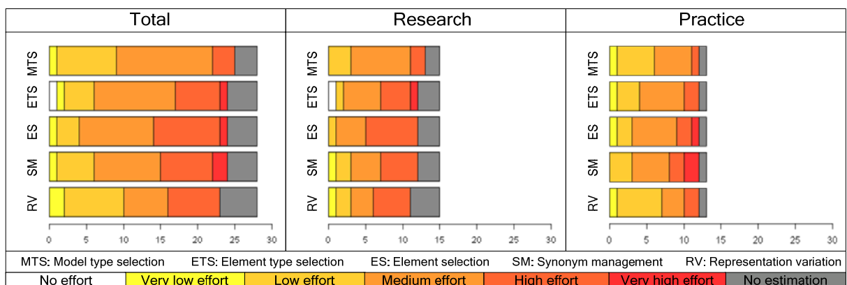
Figure 4: Effort estimation
