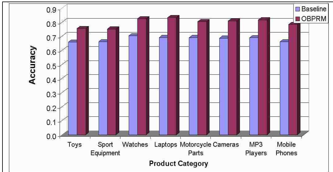
Figure 3. Comparative Performance Between OBPRM and the Baseline
