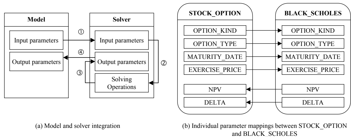
[Figure 4] Model and Solver Integration Scheme
