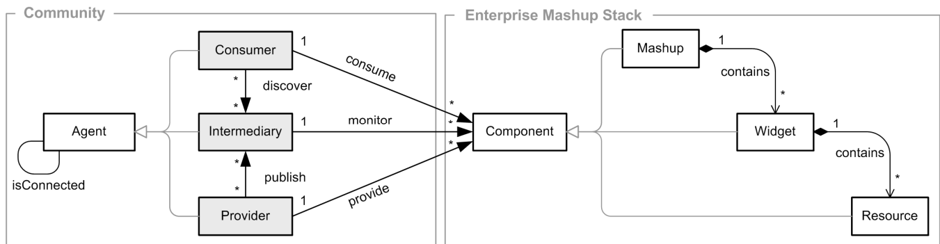
Figure 3. Interaction Agent Model for Enterprise Mashups
