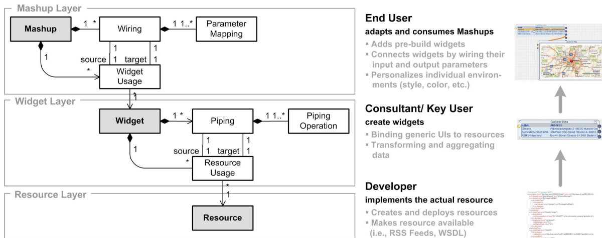
Figure 2. Enterprise Mashup Stack – Meta Model and User Roles (Hoyer and Stanoevska-Slabeva, 2009).
