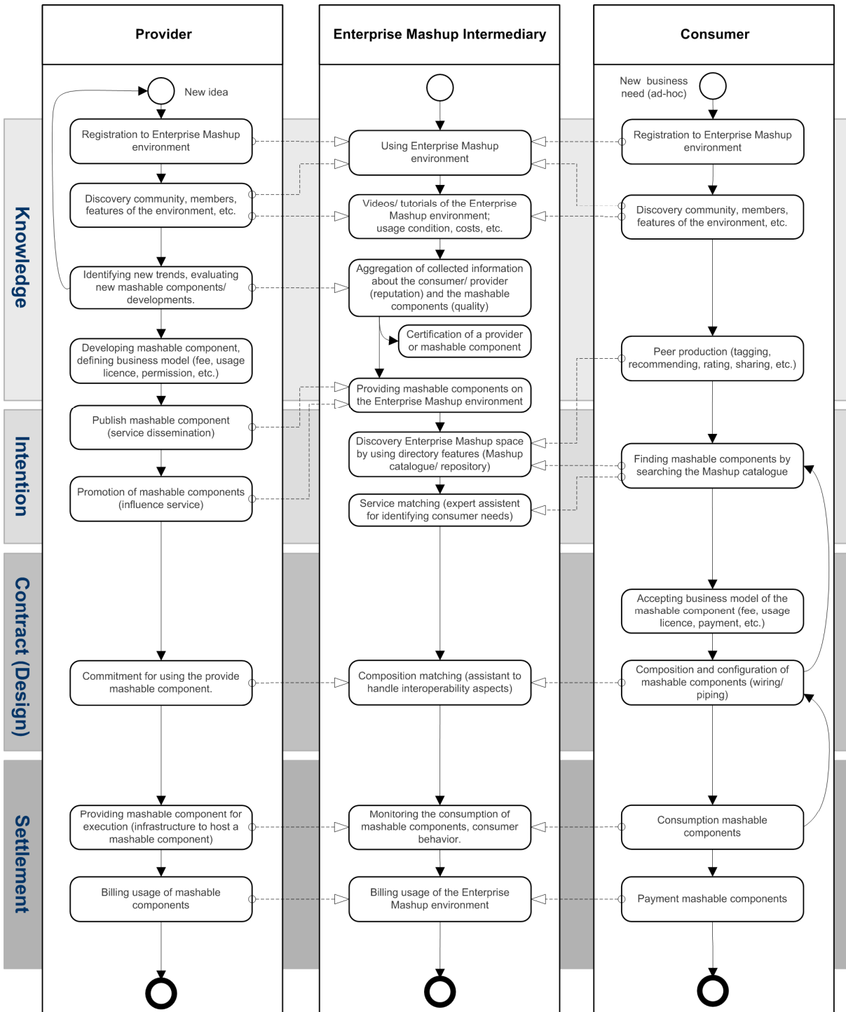
Figure 4. Interaction Phase Model and Features of Enterprise Mashup Intermediaries
