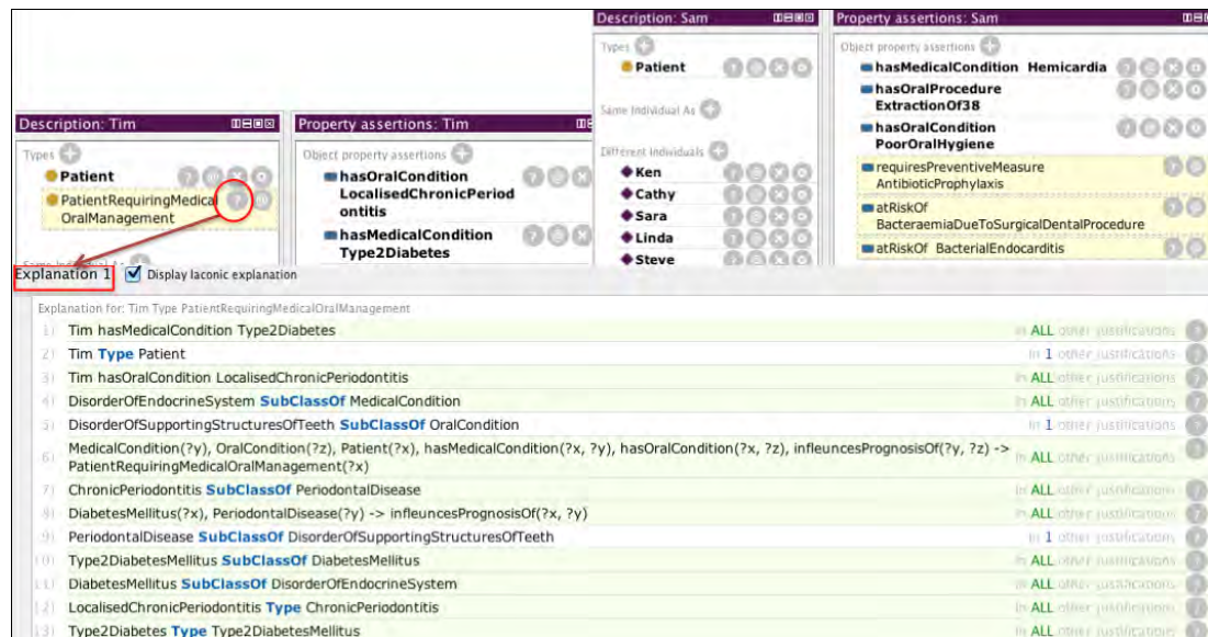
Figure 3: Snapshot of example inferencing outputs and reasoning justification in Protégé
