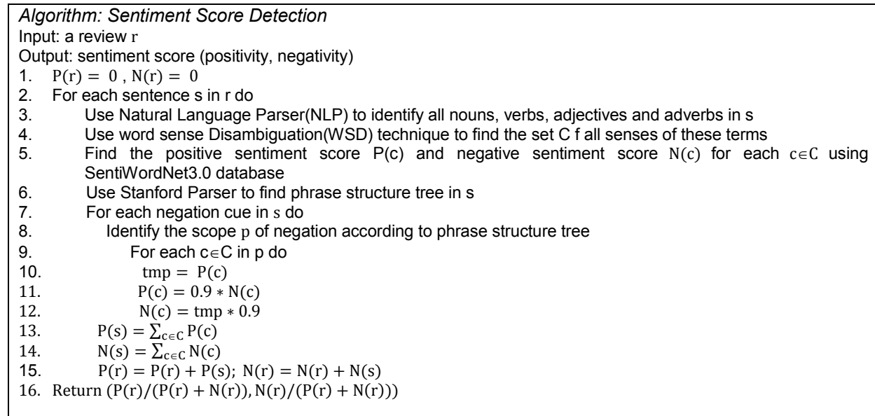
Figure 3 - Algorithm for sentiment score detection
