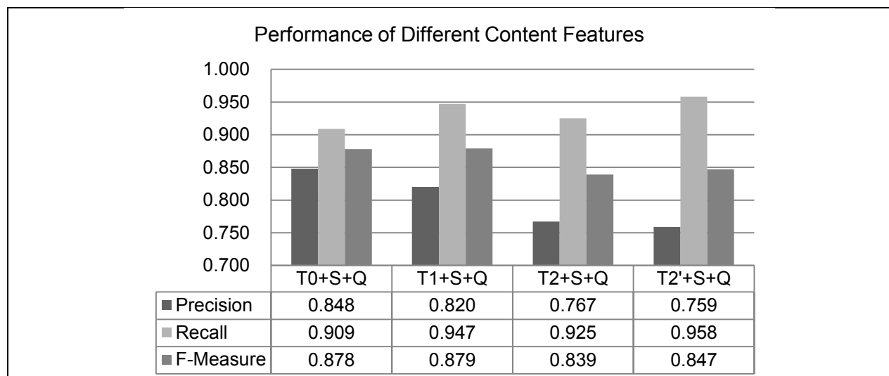
Figure 6 - Performance of different methods for representing content features
