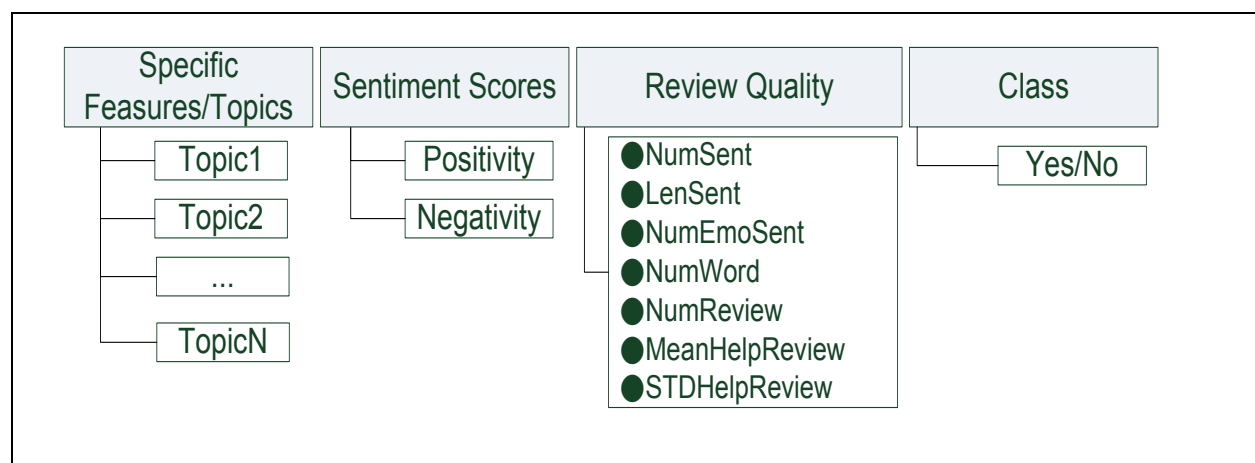
Figure 4 - Representations of reviews
