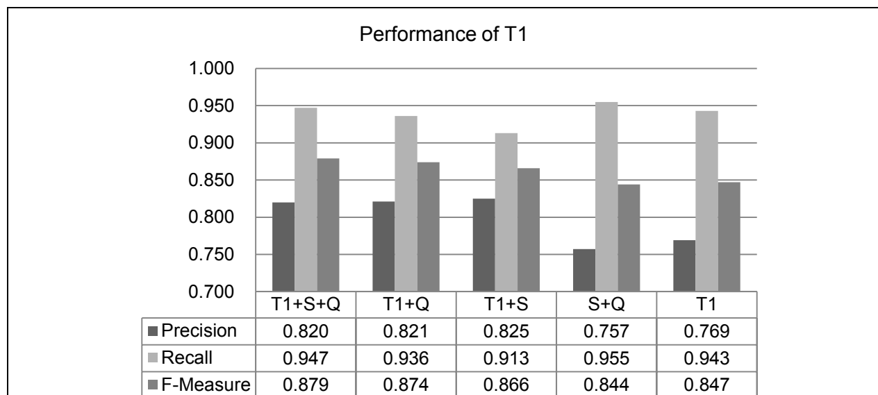
Figure 7 - Performance of different combinations of T1, S, and Q
