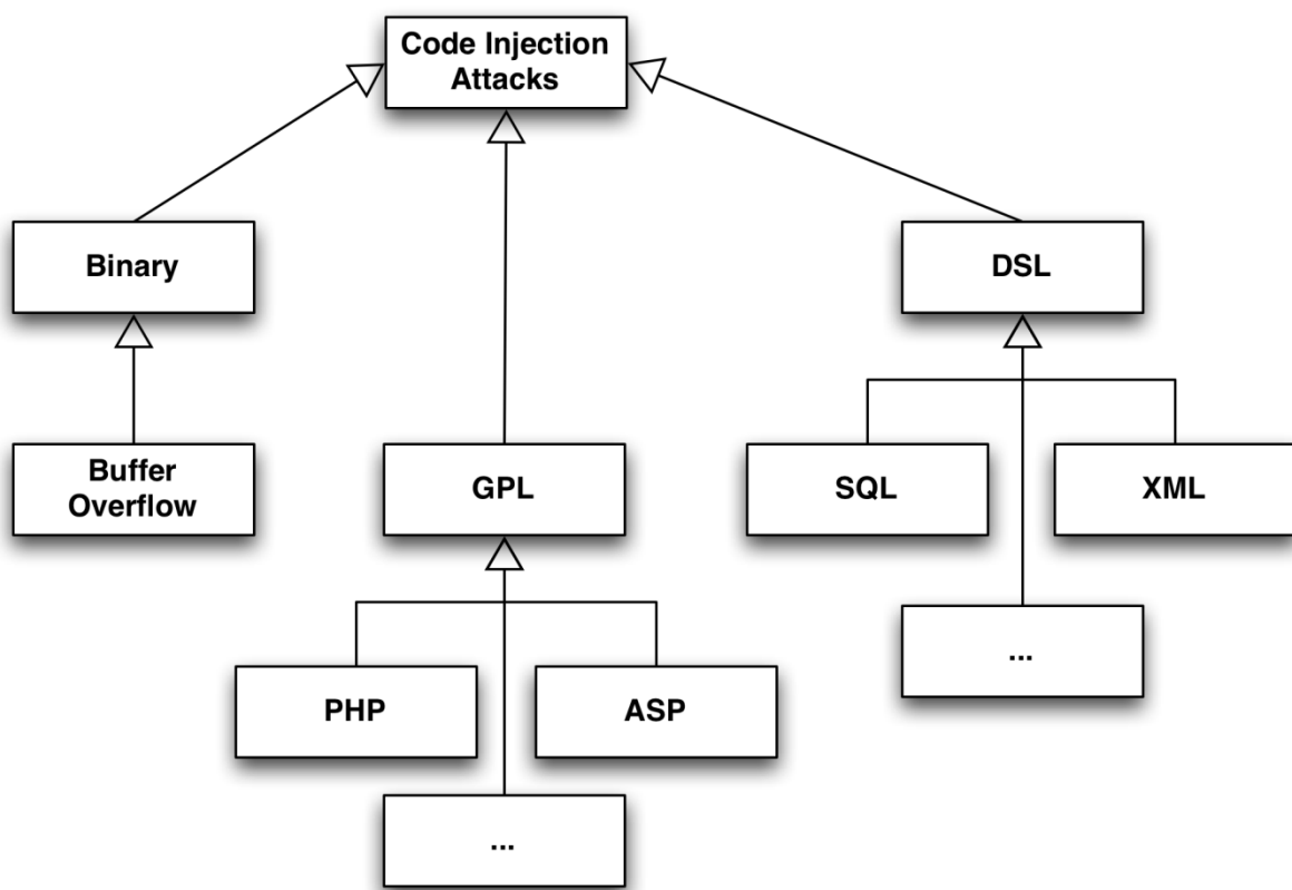
Figure 1 A taxonomy of code injection attacks
