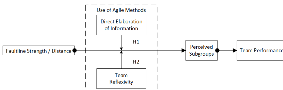
Figure 2. Hypothesized interaction of constructs. Source: Own figure.
