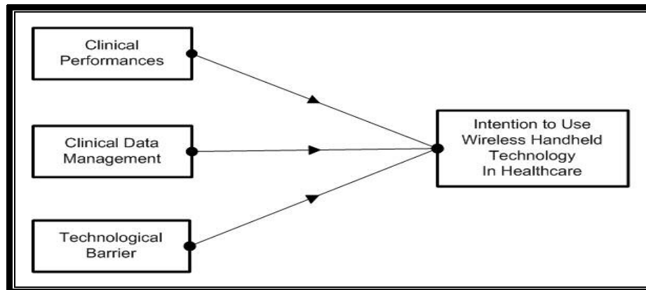
Figure 1: Research Model
