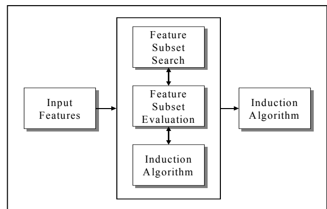
Figure 2 Process of a generic wrapper model
