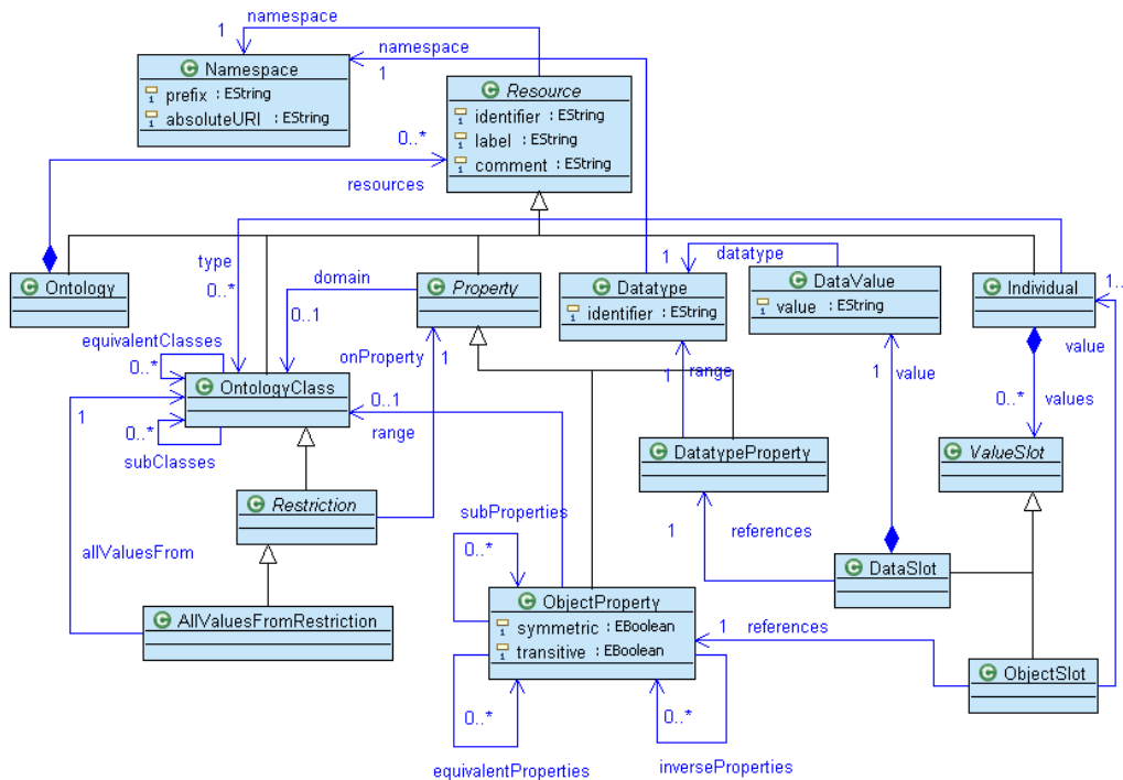
Figure 2 Lightweight Ontology Metamodel
