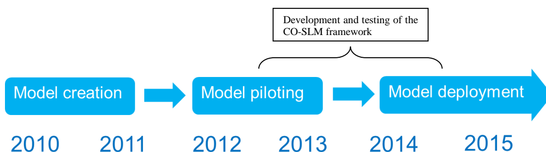
Fig. 2. Timeline for the development of the CO-SLM model
