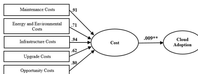
Figure 3: Structural equation model (SEM) test
