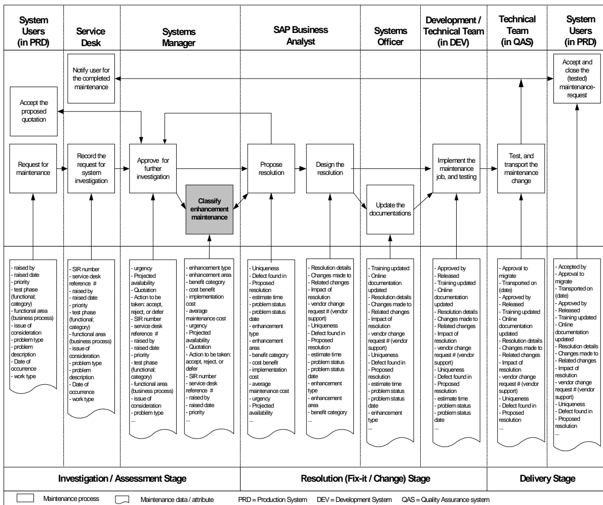
Figure 2: The proposed maintenance-data-model for ERP maintenance
