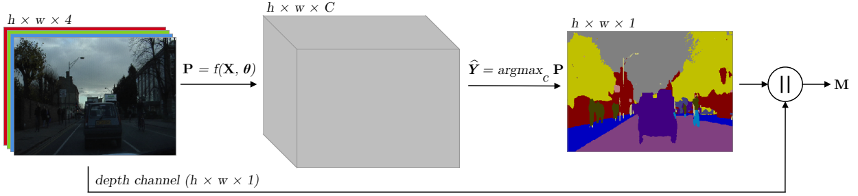
Figure 1. The perception task is modeled as a Convolutional Neural Network (CNN) f(x, \theta) : \mathbb{R}^{h \times w \times 4} \rightarrow \mathbb{R}^{h \times w \times C} , where C is the number of labels in the classification task. An RGB-D input tensor \mathbf{X} passes through the CNN to generate a probability tensor \mathbf{P} = f(\mathbf{X}, \theta) . For each pixel, the label with the highest probability is taken as the predicted label, i.e., \hat{Y} = \arg \max_{c \in C} \mathbf{P}_{:, :, c} . The depth channel, \mathbf{X}_{:, :, 4} , is concatenated with the predicted targets, \hat{Y} , to produce a 3-dimensional semantic map \mathbf{M} .
