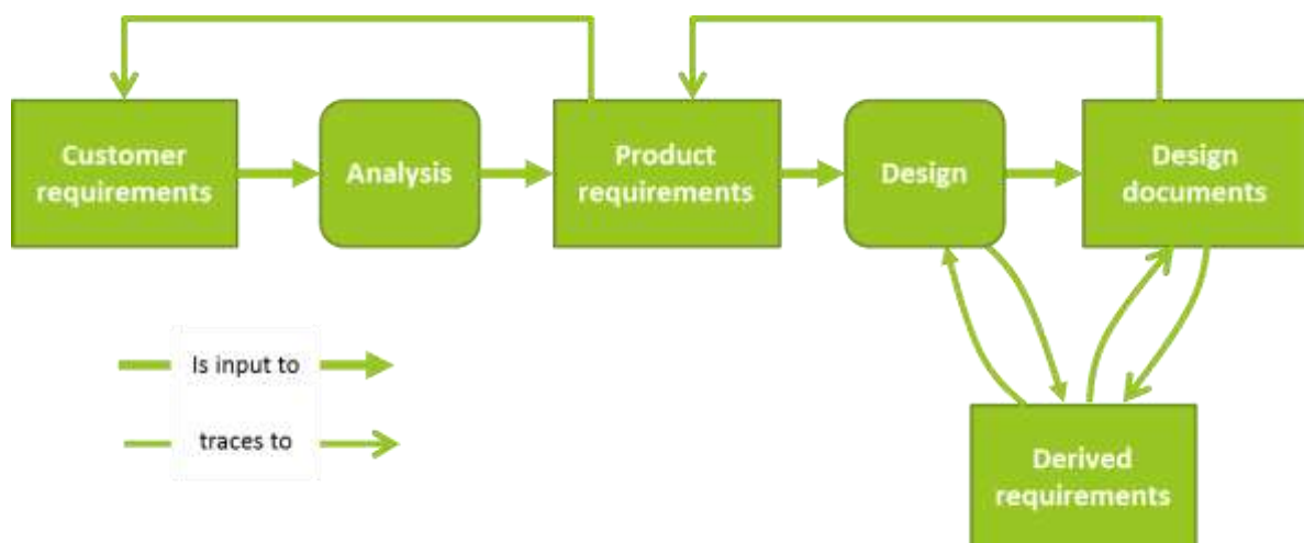
Figure 1: Requirement types (Brooksby, 2003)
