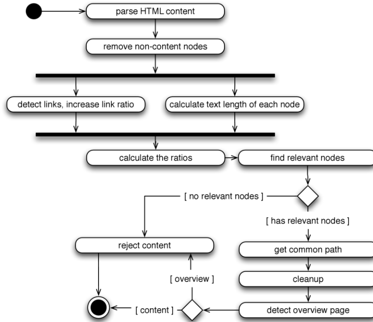
Figure 2. Activity diagram of the TextSweeper HTML pre-processing component
