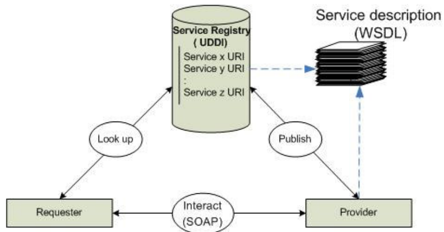
Figure 1: Web Service Architecture
