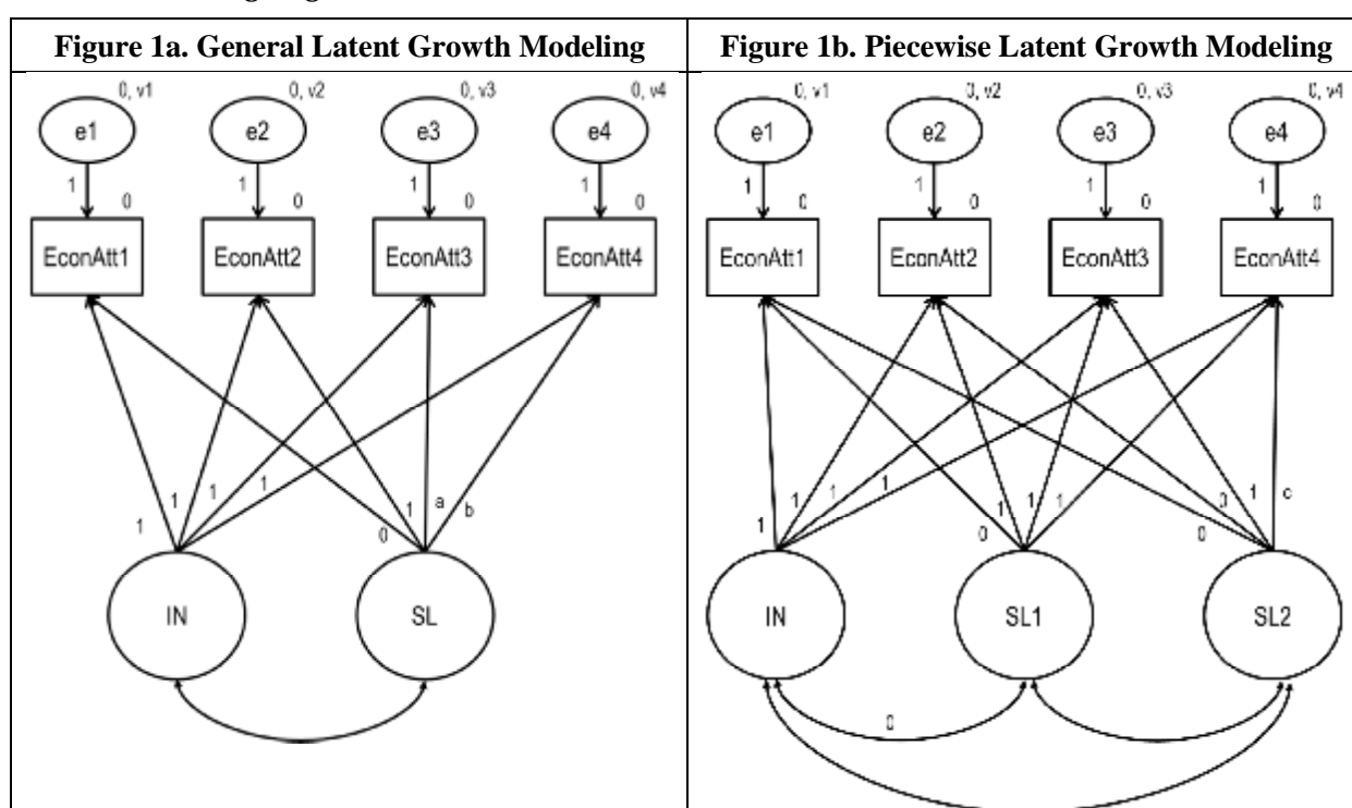
Note: IS – Intercept, SL – slope, EconAtt – economic attitude In Figure 1b, the covariance between IN and SL1 is set to zero for identification purposes.
